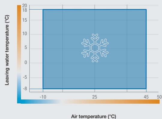
Full load operating limits
